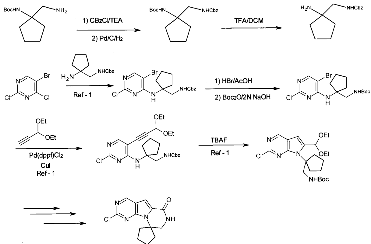
Scheme 2
